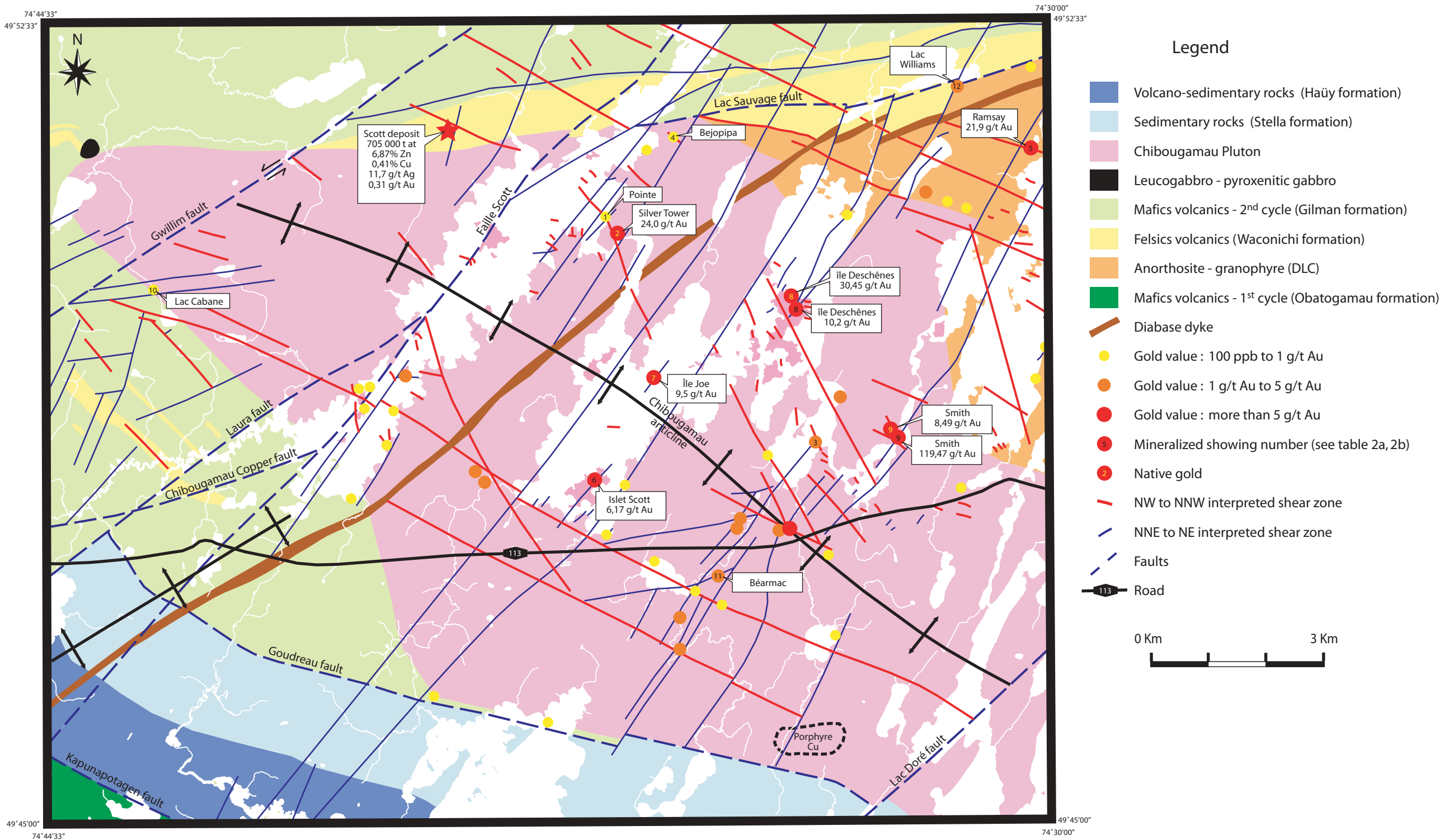
Figure 2 - Detailed geology of Chibougamau pluton - West part (32G/15)
