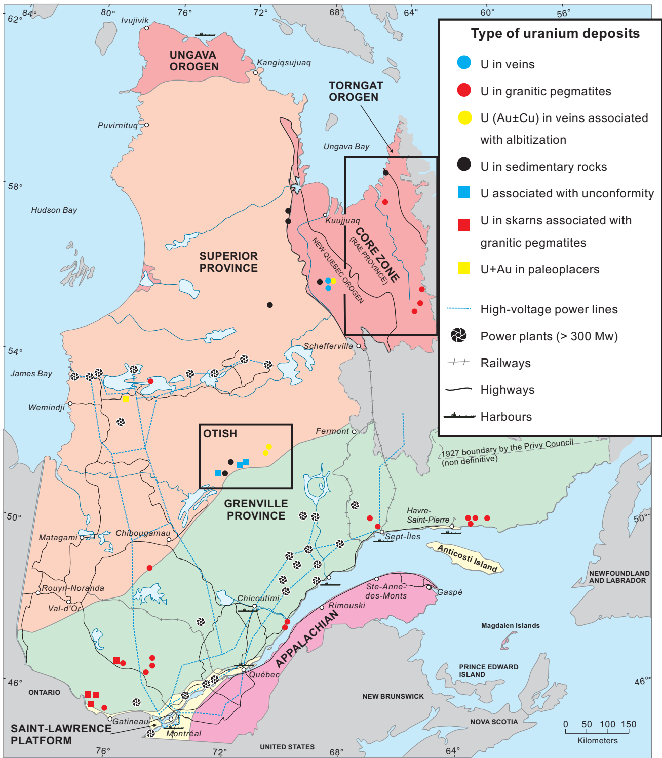
Figure 1. Geological subdivisions and distribution of the most significant uranium showings and deposits in Québec and location of the two areas of interest discuss in the paper : the Otish Basin (OTISH) and the Core Zone.
